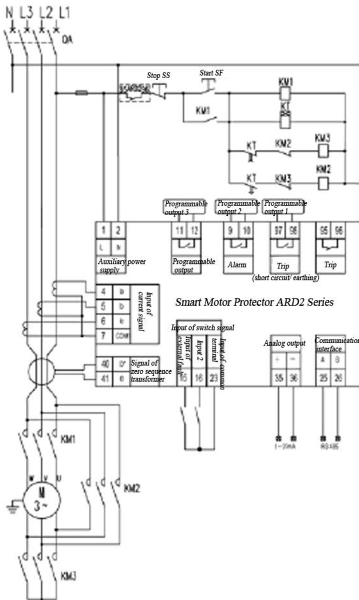
Y-Δ Start Wiring of Motor Protector ARD2
