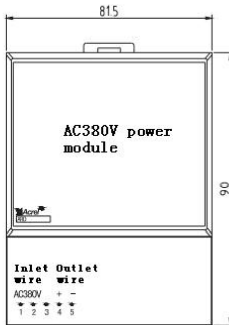
Figure 9 Outline dimensions of AC380 power module
